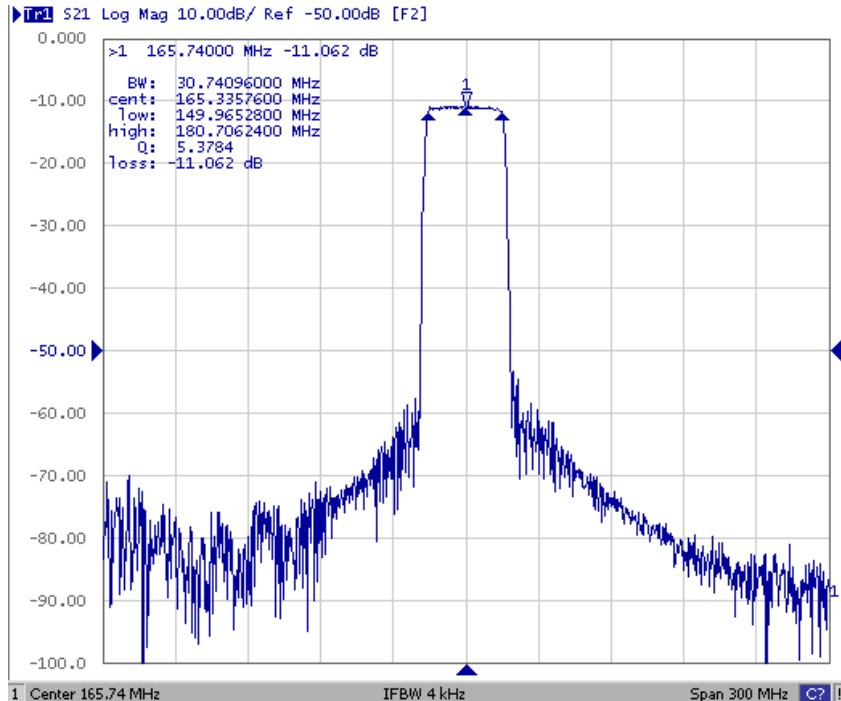
Fig. 1. Horizontal: 30MHz / Div, Vertical: 10dB / Div
